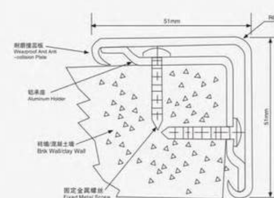
扶手安装说明图 installation of handrail
