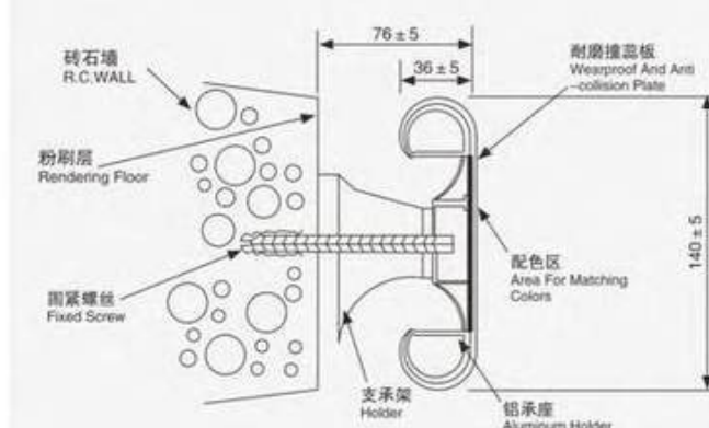
扶手安装说明图 installation of handrail
